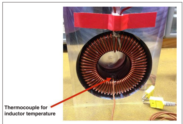
Figure 3: Detail showing the thermocouple location on the inductor, on the inner edge of the toroid opposite the wire leads.
