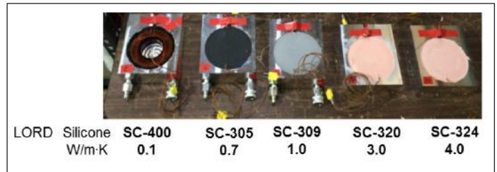
Figure 2: Inductors potted in aluminum cooling plates with each of the LORD potting materials.
