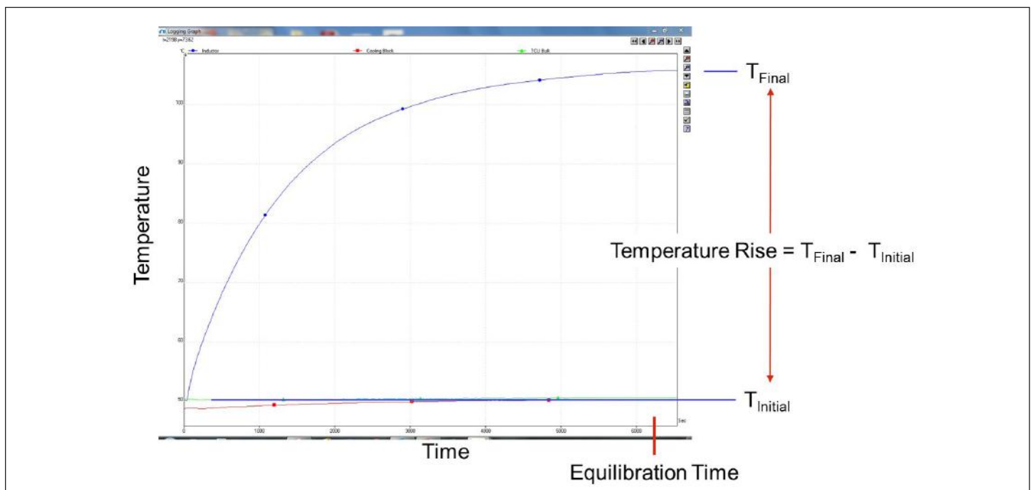
Figure 5: Temperature profile for a typical Thermostet SC-400 encapsulant potted inductor test, showing definitions of temperature rise and equilibration time. The blue line is the inductor, and the nearly-horizontal red line is the cooling plate.
