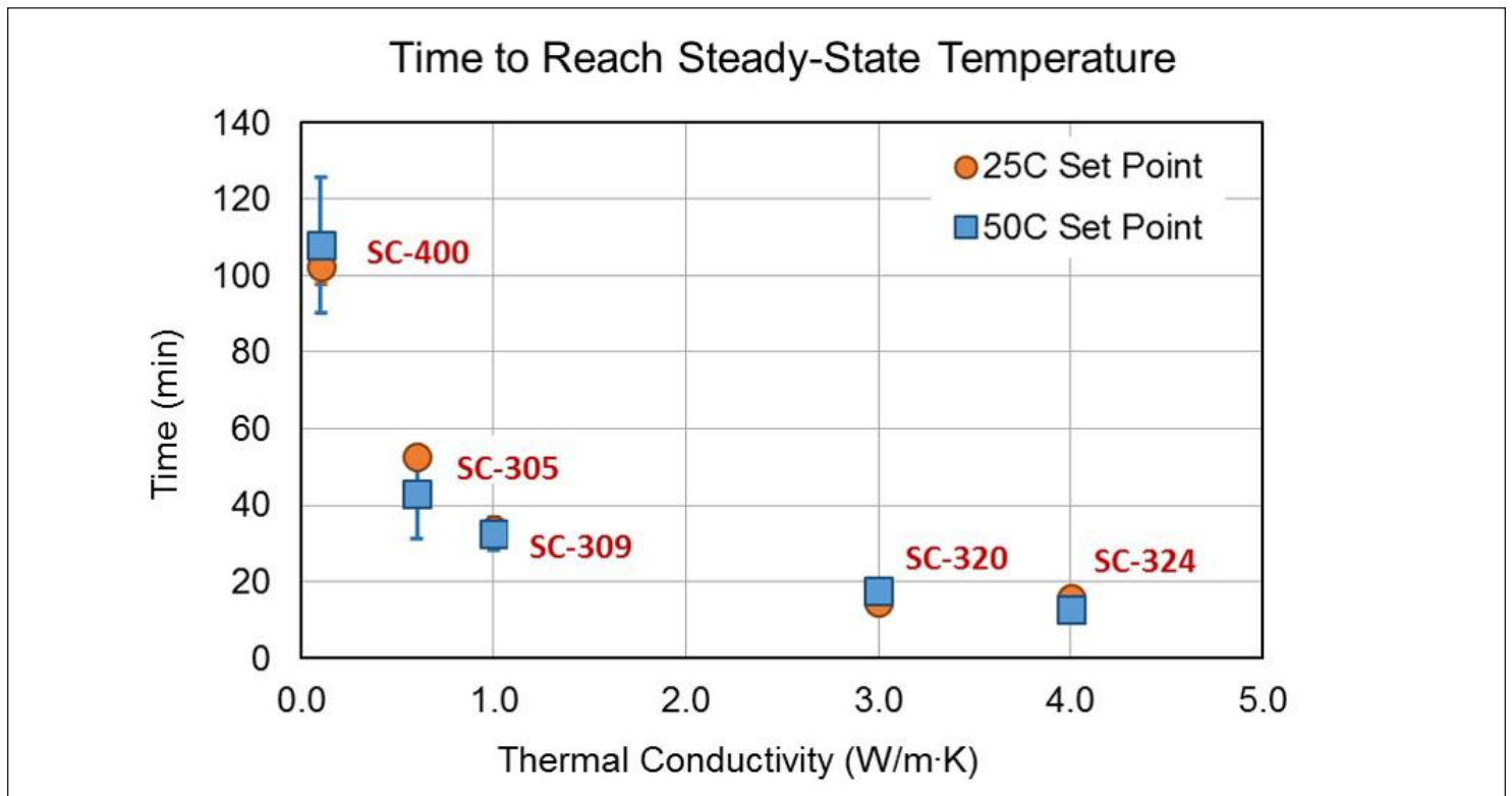
Figure 7: Average time to reach steady-state temperature (equilibration time) for inductors in the study at both 25°C and 50°C set points of the liquid coolant.
