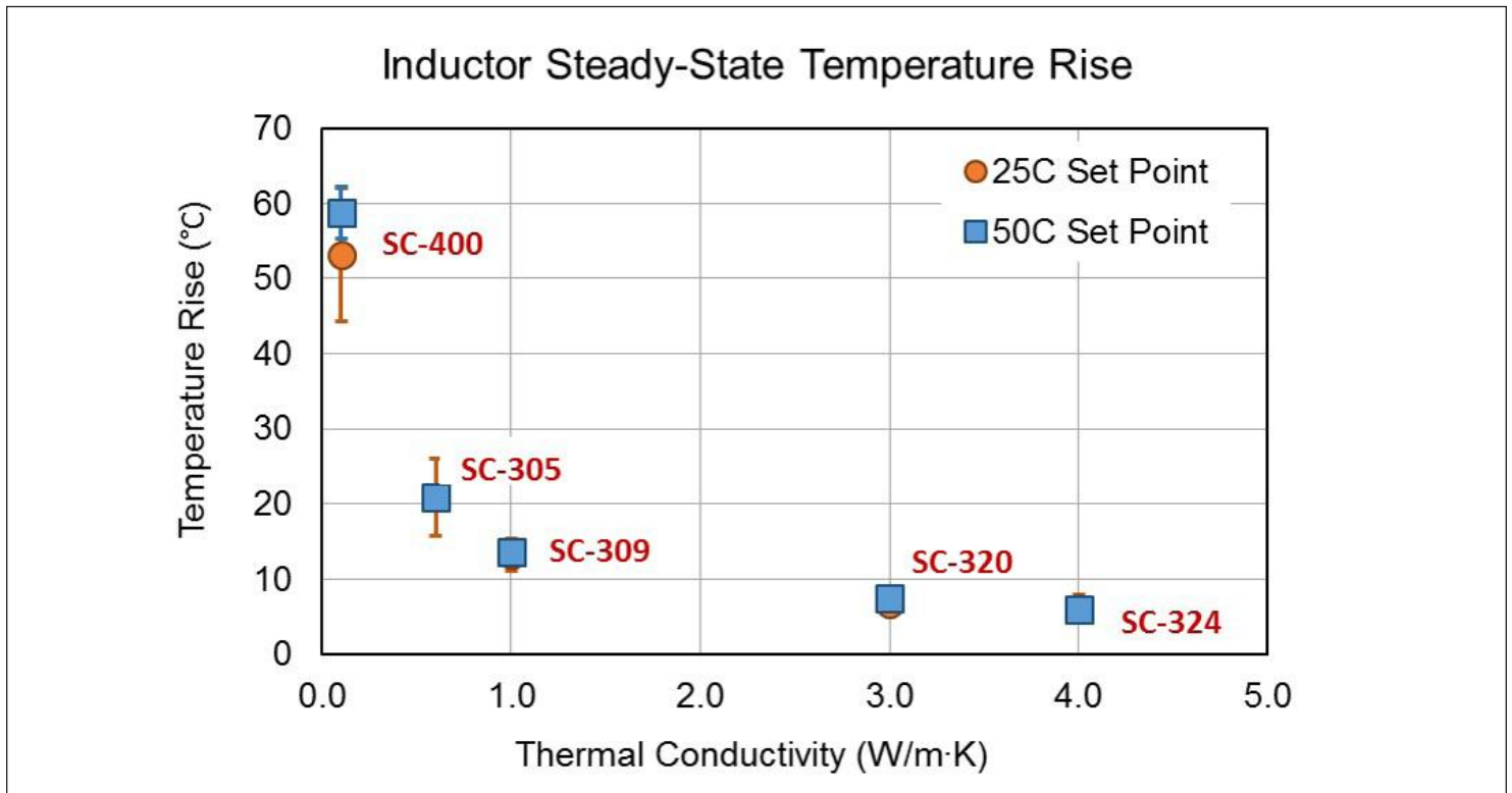
Figure 6: Average temperature rise for inductors in the study at both 25°C and 50°C set points of the liquid coolant.
