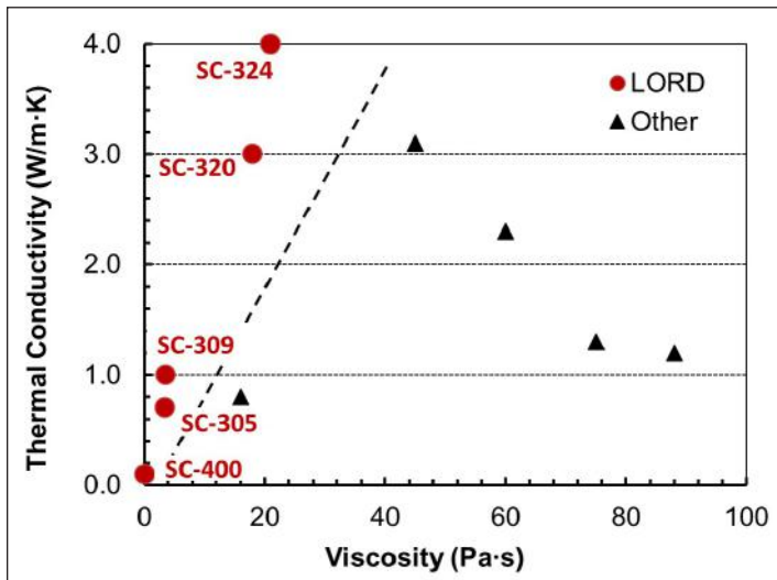
Figure 1: Thermal conductivity versus viscosity for various potting materials. Commercially-available LORD materials are indicated as red circles.
